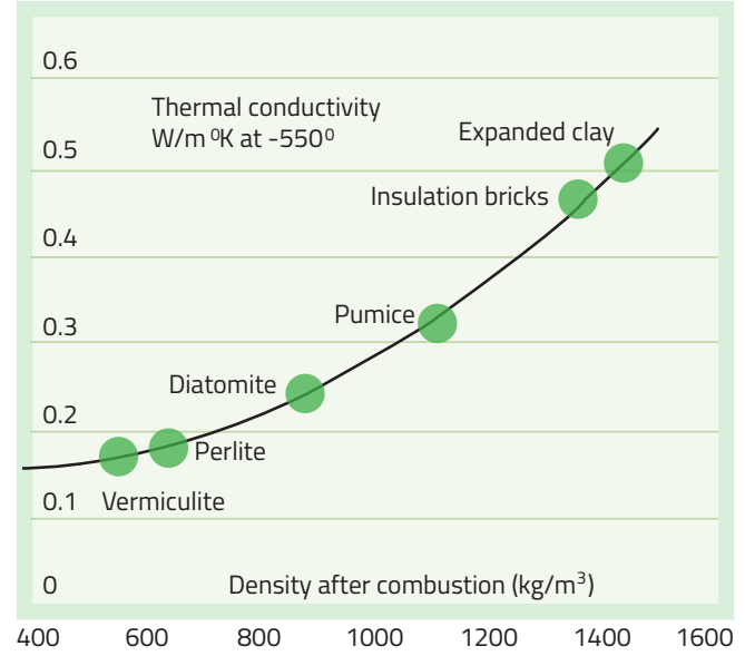
Figure 3: The relationship between the thermal conductivity and the density after incineration of heat-resistant insulating concretes.
