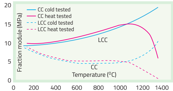
Figure 5. Fraction module of ordinary and LCC concrete.
