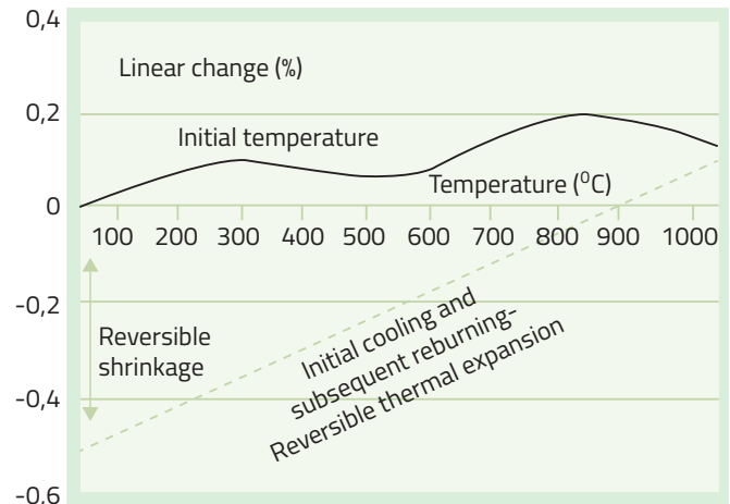
Figure 4: Heating and cooling cycle of concrete
